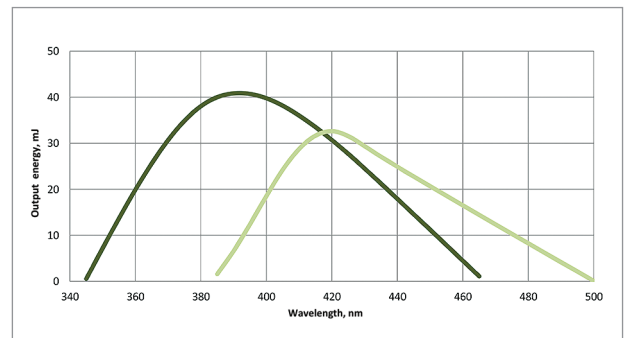
LX329A laser typical efficiency curve at second harmonic.
